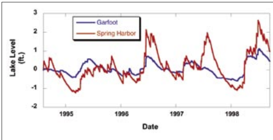
Figure 5. Lake Mendota water levels simulated for natural (Garfoot Creek) and totally developed (Spring Harbor) watershed land use scenarios. Graph: K. Potter, UW-Madison.
