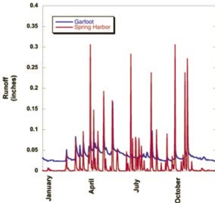
Figure 4. Water discharge from Garfoot Creek and Spring Harbor storm sewer in 1995. Graph: K. Potter, UW-Madison.
