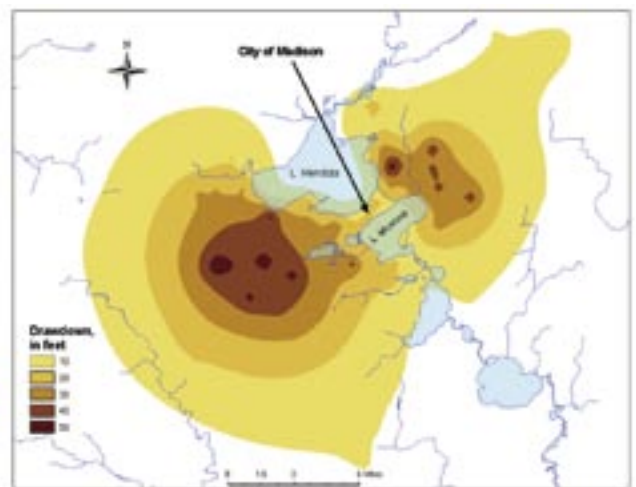
Figure 3a. Drawdown of deep aquifer near Madison. Graph: K. Bradbury, Wis. Geol. Nat. Hist. Survey.
