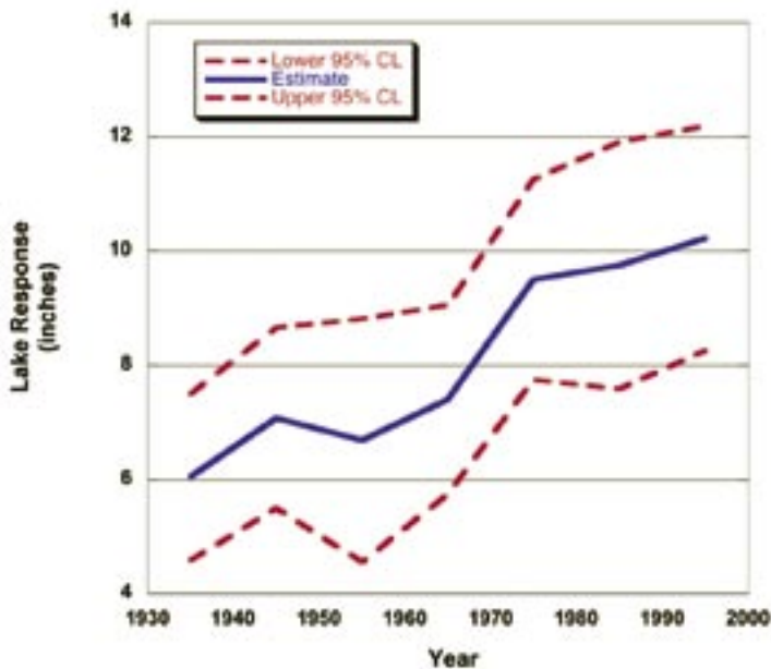
Figure 6. Decadal trends of Mendota's lake level response to six-inch rainfall events. Graph: M. Wegener and K. Potter, UW-Madison.
