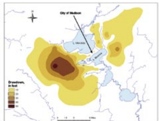
Figure 3b. Drawdown in the shallow aquifer near Madison. Graph: K. Bradbury, Wis. Geol. Nat. Hist. Survey.
