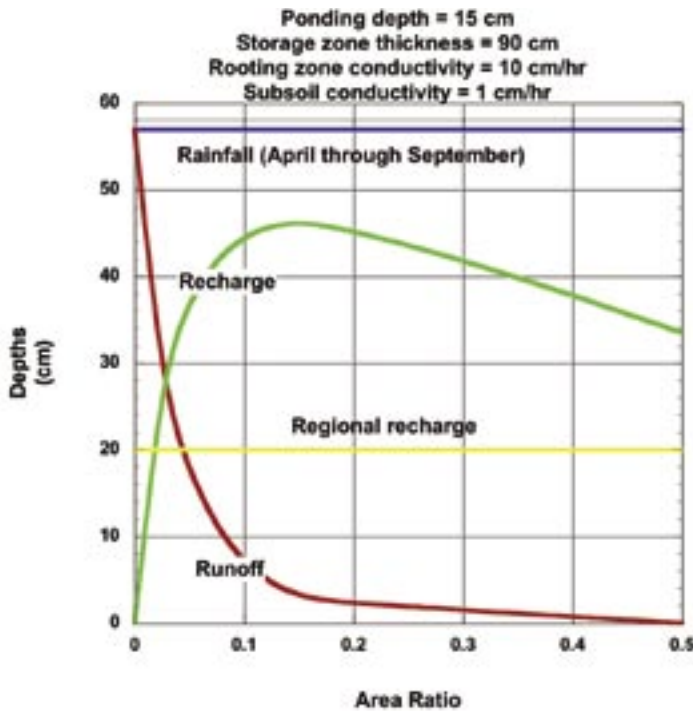
Figure 10. Rain garden simulation, 1992-1997 (from Dussailant et al. 2004).
